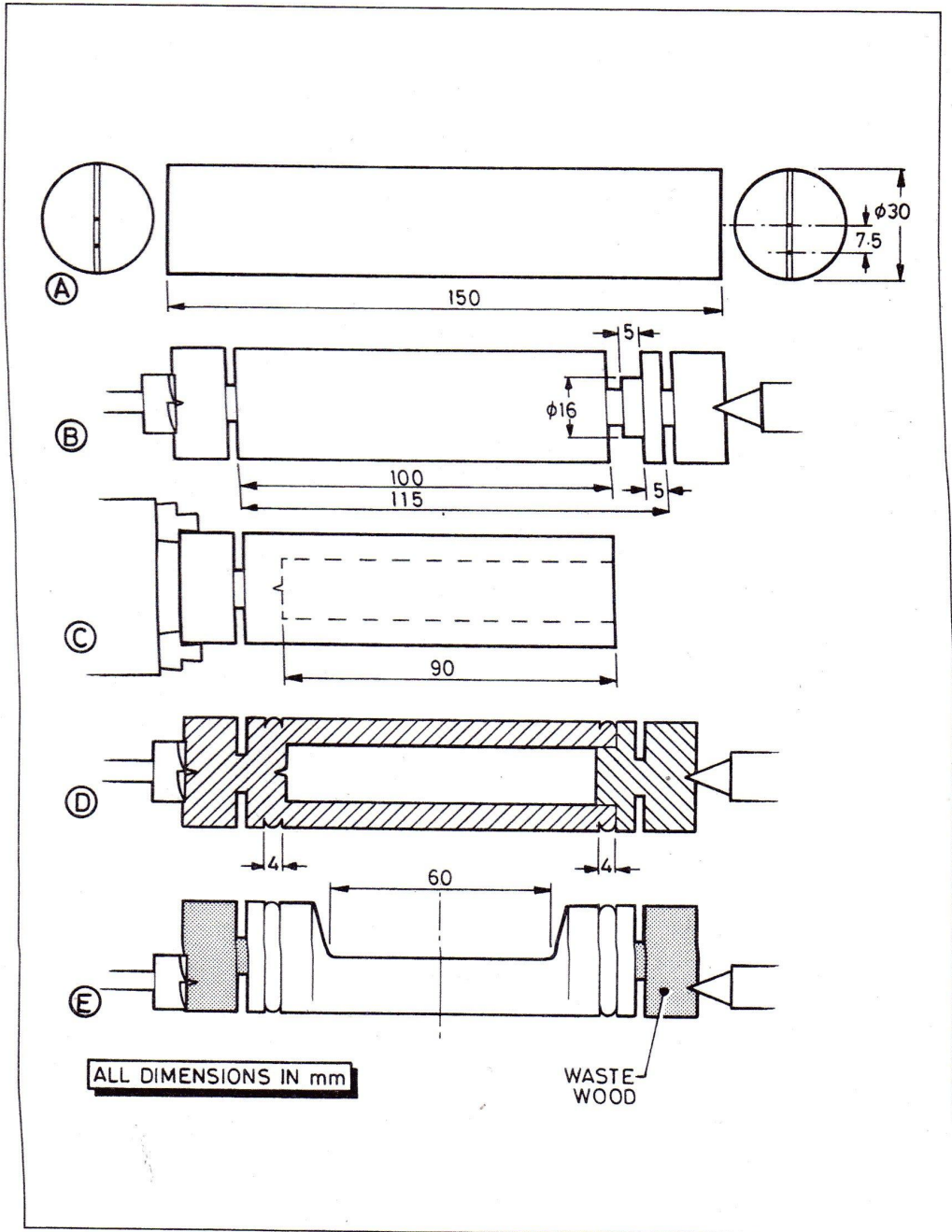
Fig 6.2 Method sequence.
